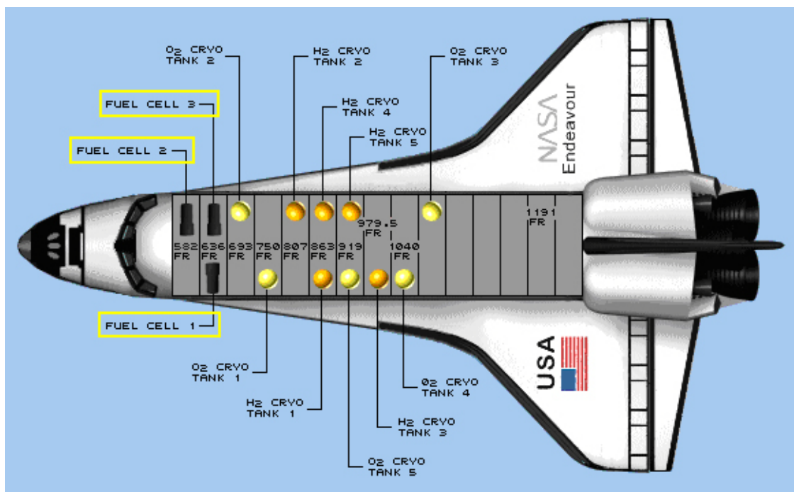
Figure 1: Typical space shuttle cryogenic tank layout
