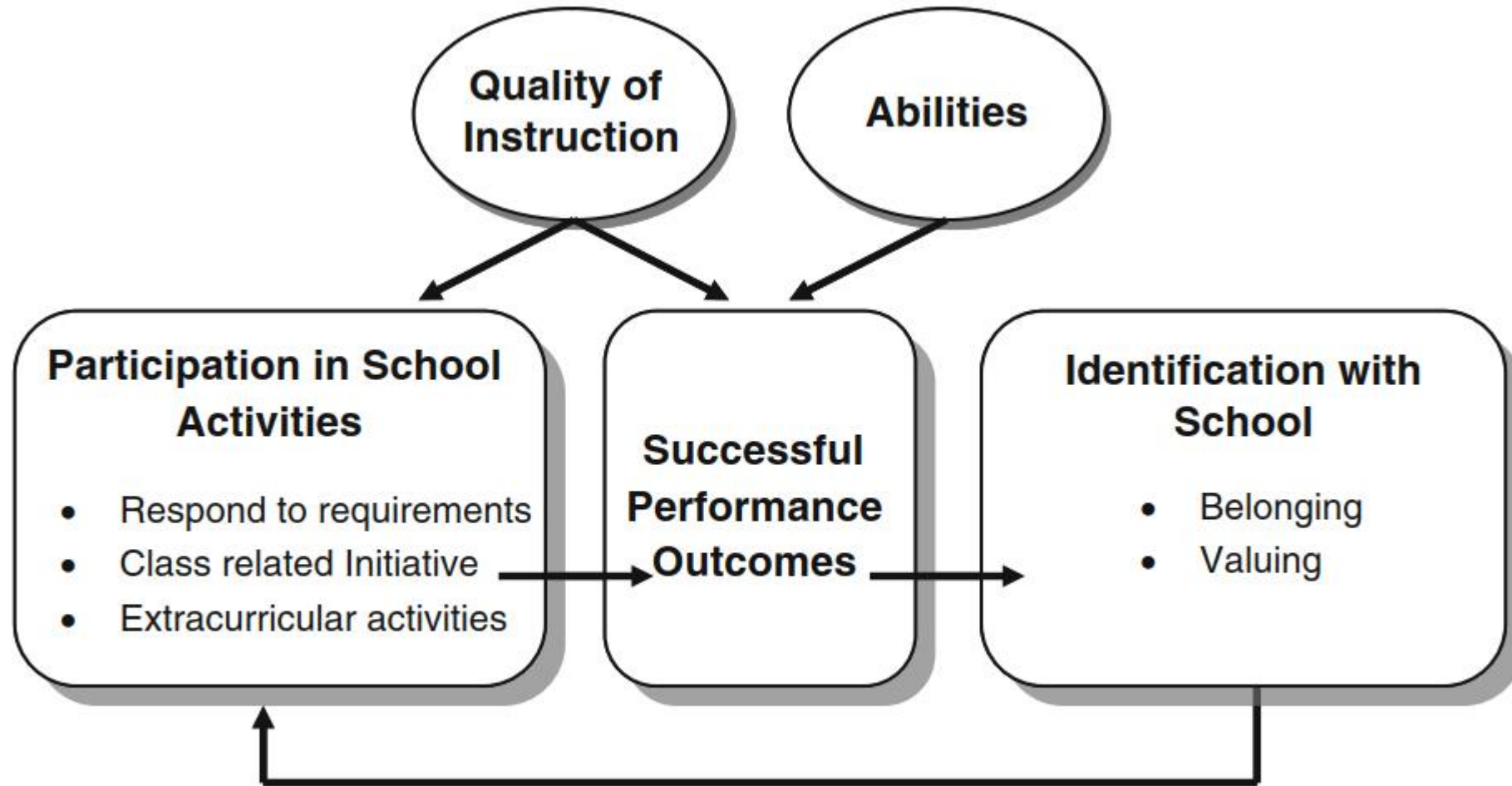
Participation-identification model
